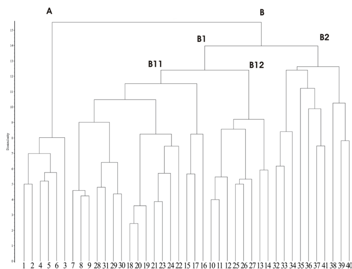
Fig. 2 - Cluster analysis (UPGMA euclidean) (41 random relèves).
